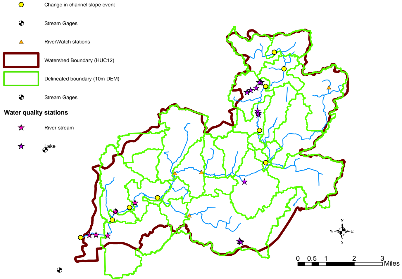
Figure 3. Delineation of subwatersheds (calculation points)
