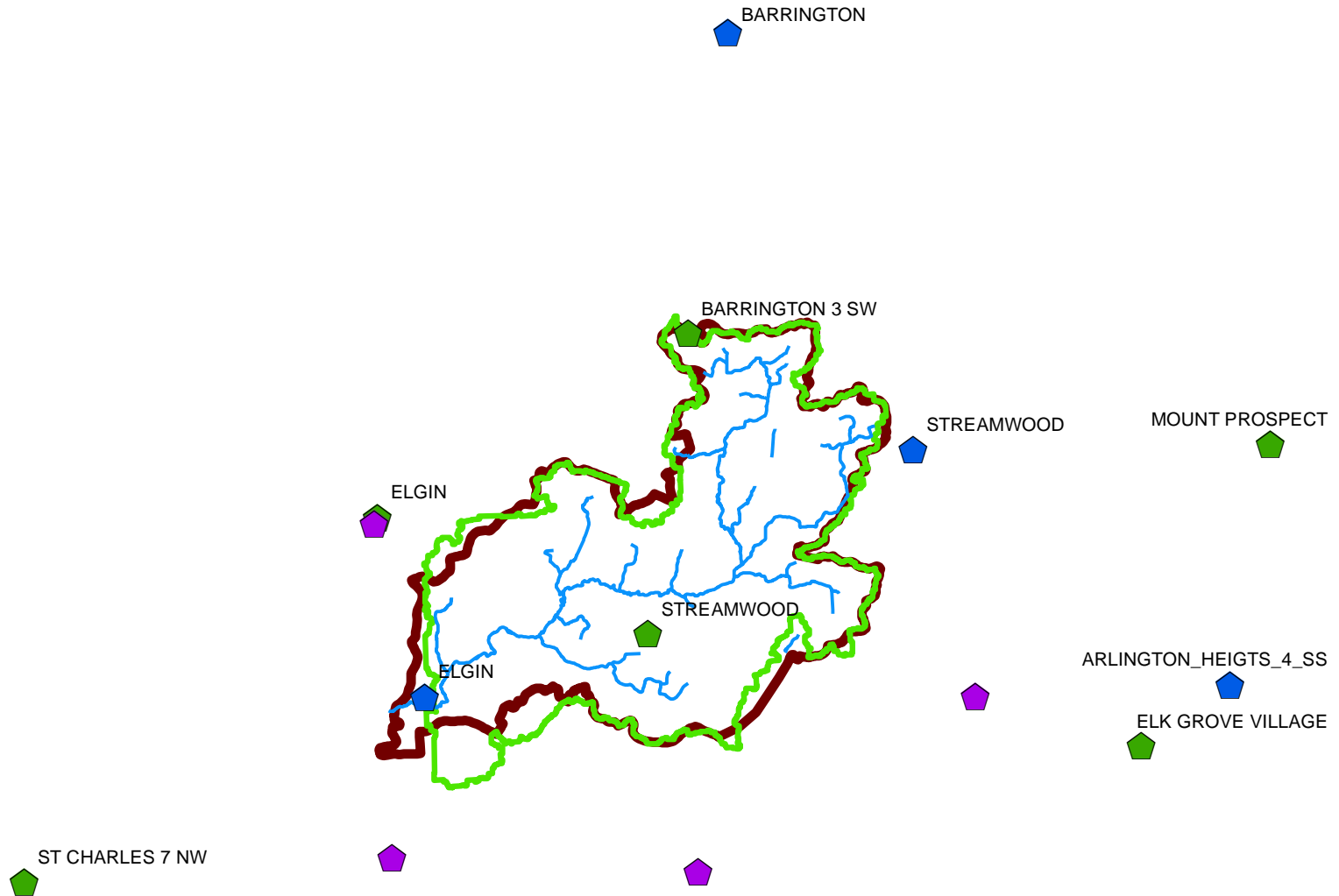
Figure 2. Location of climate stations
